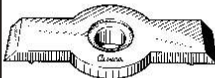
15813 (4005714) Nylon Window Glass Retainer AMC Eagle 1988-On UNIT PACKAGE: 25
